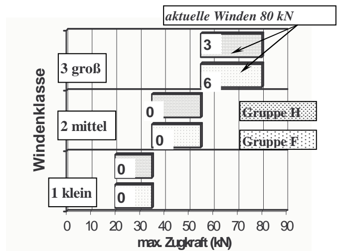
Figure: number of mounted winches tested to date Group H = lever/line controlled Group F = remote controlled Dated: November 2007
